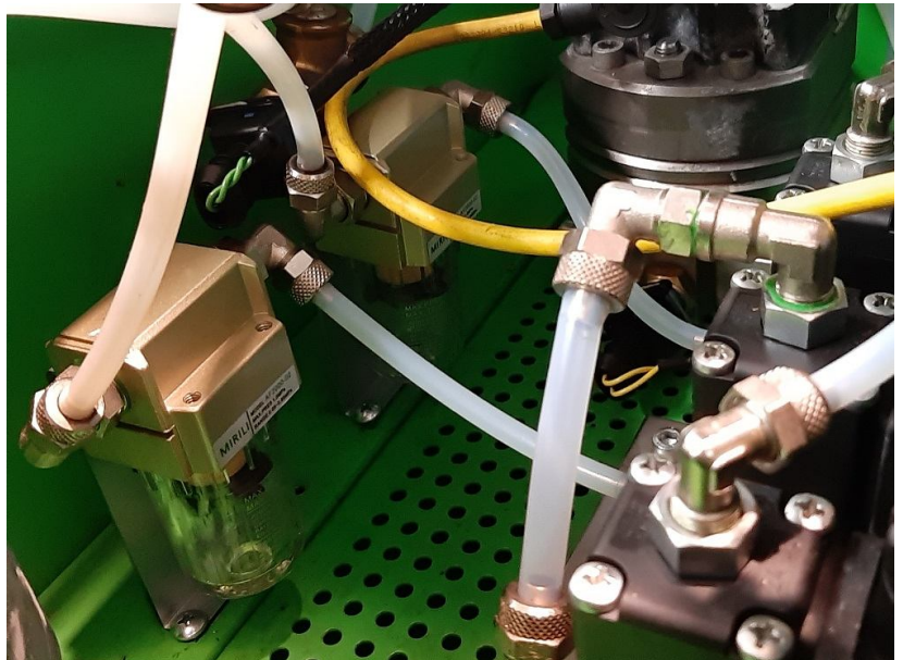
Installation example on Test bench type 555-DDP
