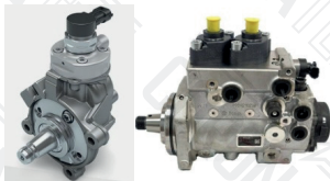
BOSCH CP425/1 - CPN5
