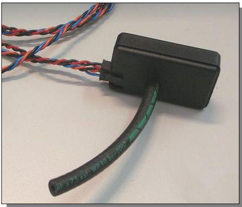
Decoder with 0-2 Bar sensor P.N.: 555-Ø2PRESS/ DEC
